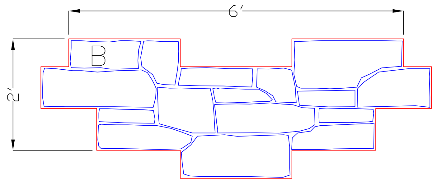
Form liner Pattern Modules
