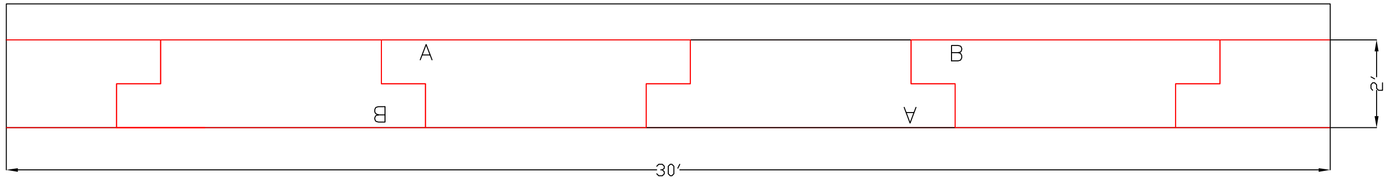
MS-2003 24" Small Ashlar Guardwall
